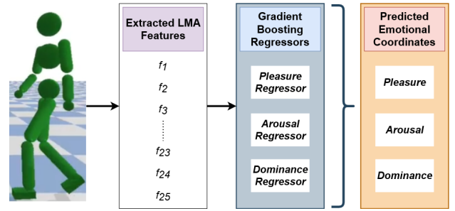
Fig. 4. The process of using our Gradient Boosting Regressors to predict the PAD coordinates of a set of LMA features extracted from a motion
