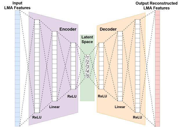
Fig. 7. The Autoencoder architecture.
