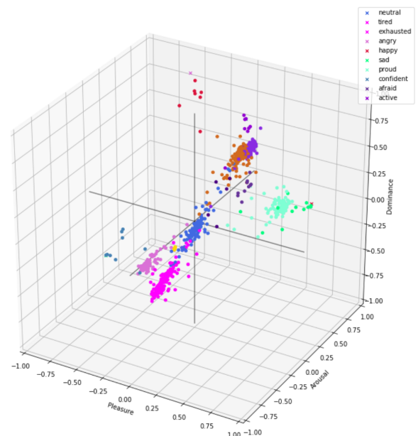
Fig. 5. Prediction results of samples from our Test set. Each sample is coloured according to their real emotion.
