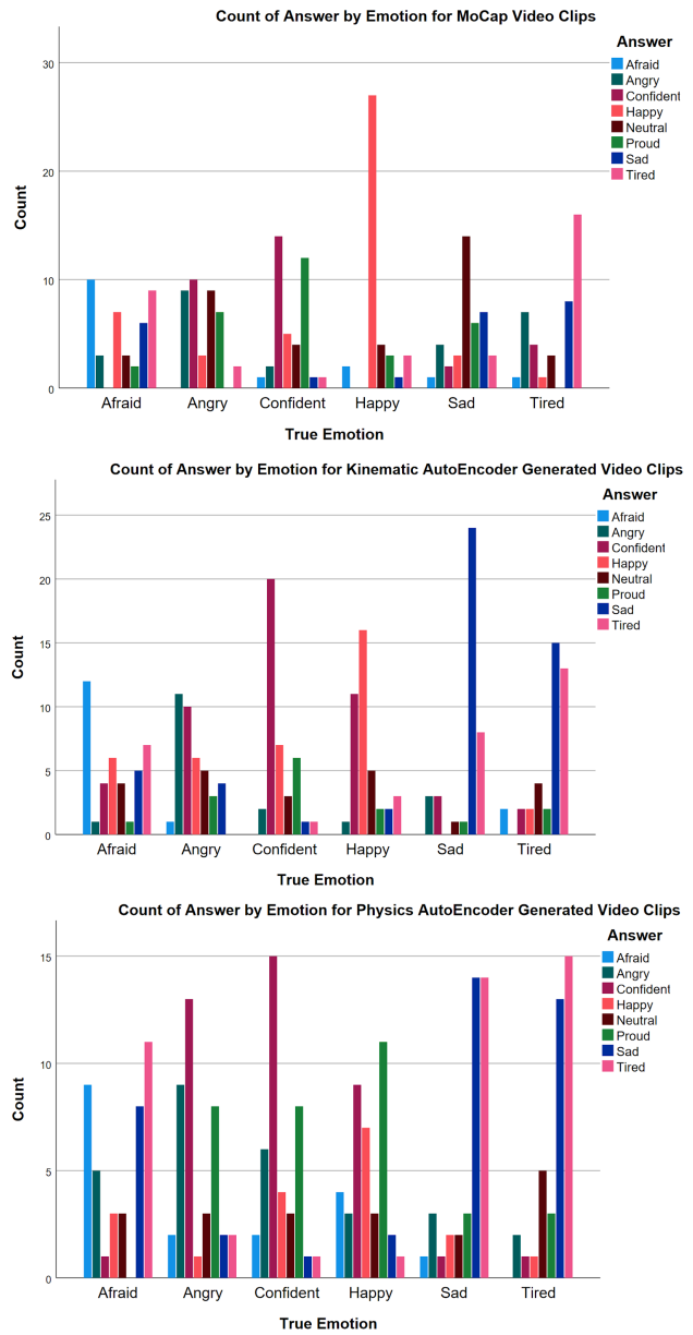
Fig. 11. Clustered bar charts showing the count of answers compared to the correct emotion for each type of clip.
