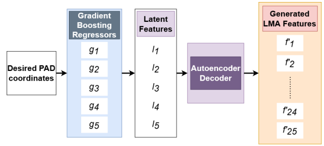
Fig. 6. Generation of LMA Features from PAD coordinates.
