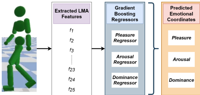
Fig. 5. The process of using our Gradient Boosting Regressors to predict the PAD coordinates of a set of LMA features extracted from a motion
