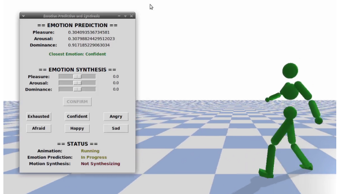
Fig. 10. Our system displaying motion capture data and our Graphical User Interface showing the current Emotional Prediction, system state and Motion Synthesis controls.
