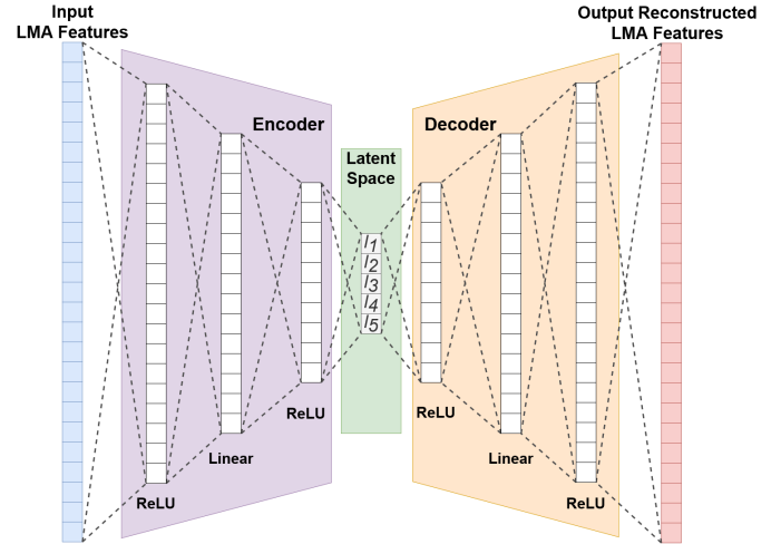
Fig. 8. The Autoencoder architecture.
