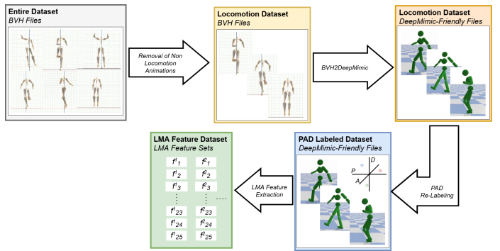
Fig. 3. The process of converting the Dataset’s BVH files into a collection of usable LMA Feature sets.
