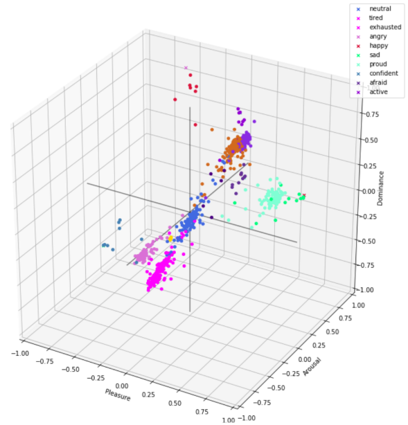
Fig. 6. Prediction results of samples from our Test set. Each sample is coloured according to their real emotion.
