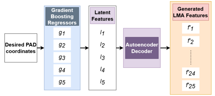
Fig. 7. Generation of LMA Features from PAD coordinates.
